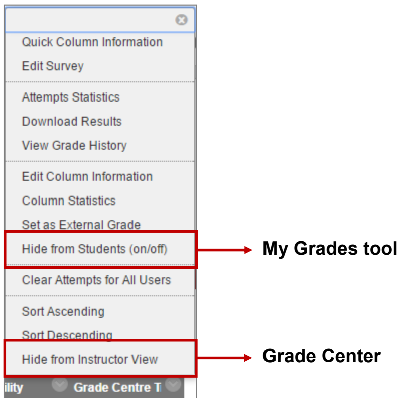
Figure 1: Column menu
